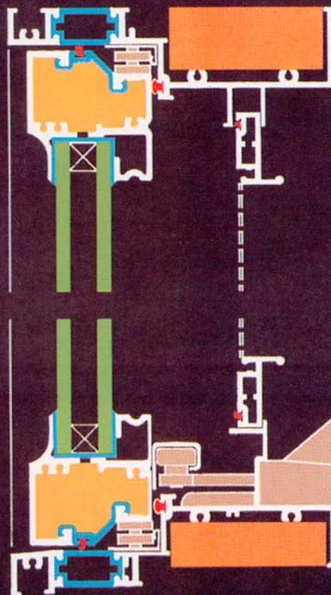
Vertical Section
