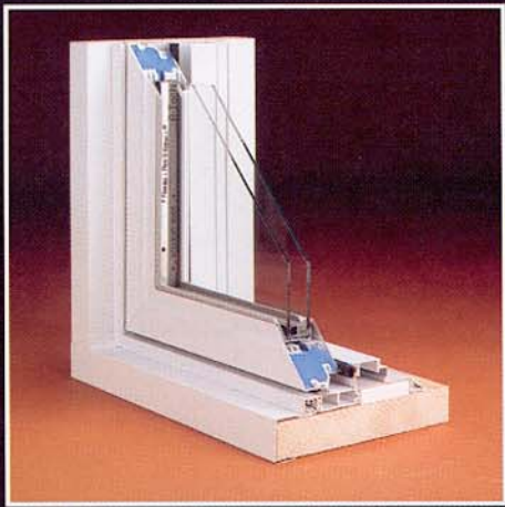
4 3 / 4 LX and pine frame with outside coating
